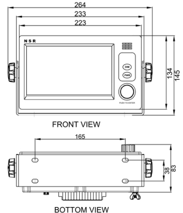
COMPASS UNIT
